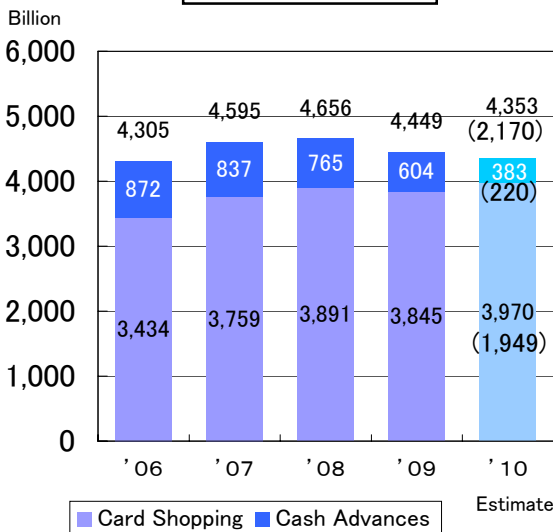
Transaction Volume
